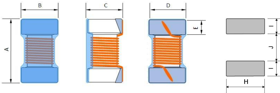
Land Pattern
